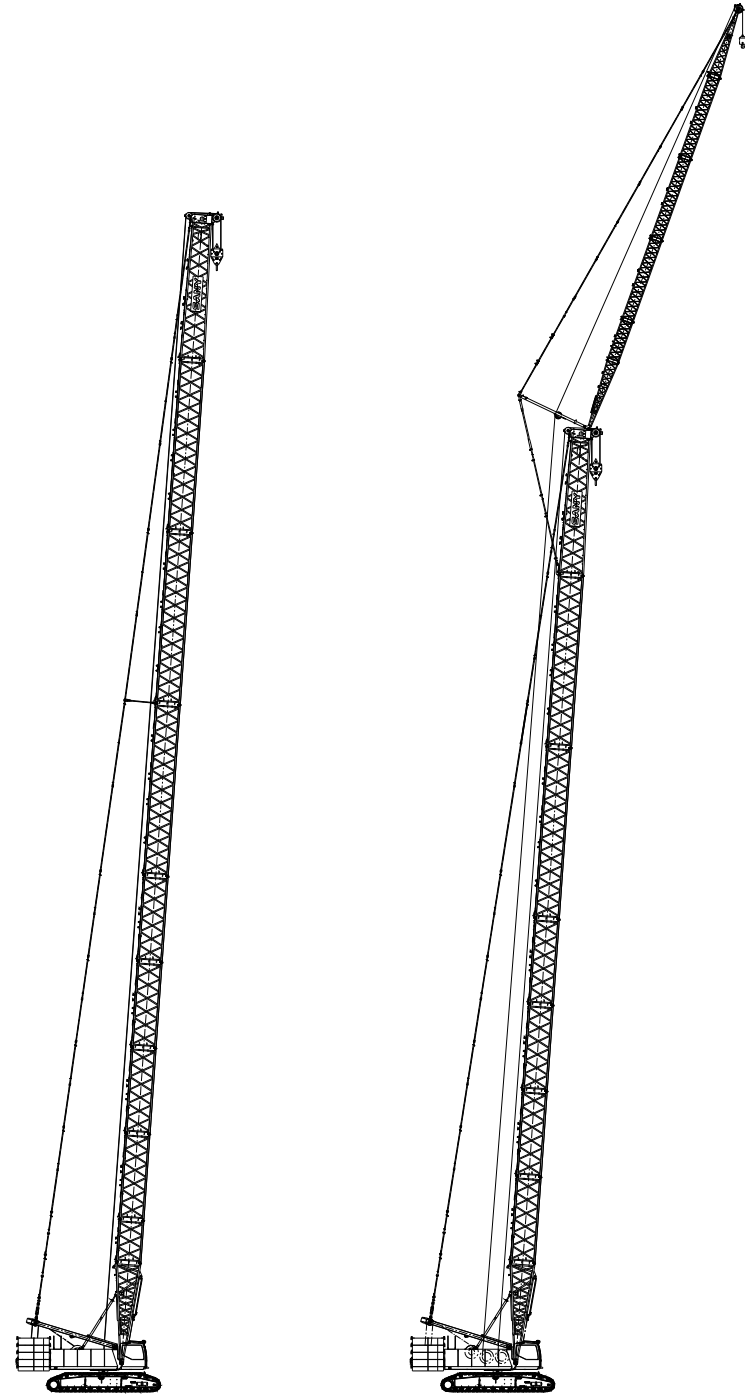
Boom H working condition
