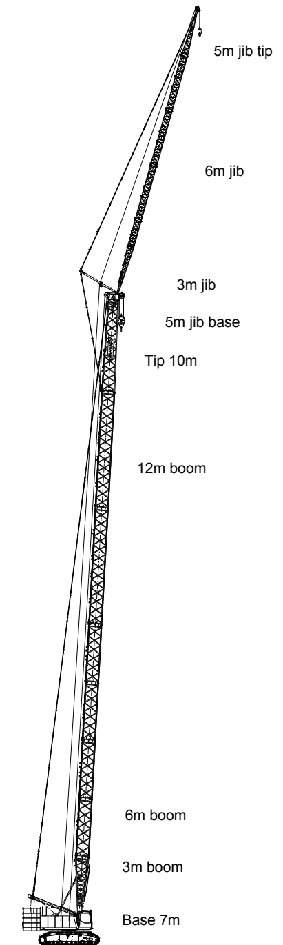
Fixed jib FJ working condition: (17m-71m) + (13m-31m)
