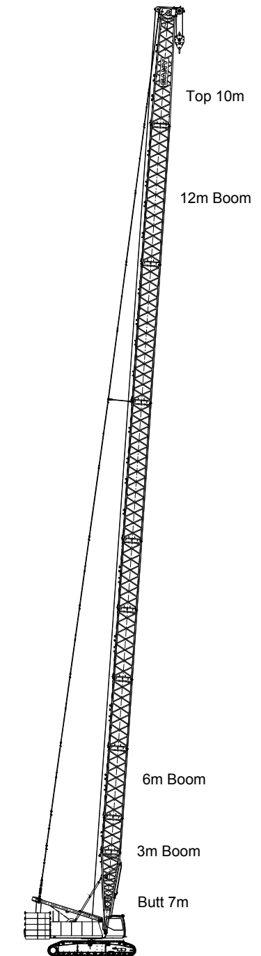
Boom H working condition: 17m-80m
